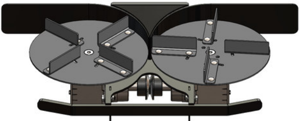
Fig 14.2.2 – Flat Vane configuration
