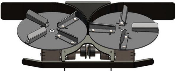
Fig 14.2.3 - Scoop configuration
